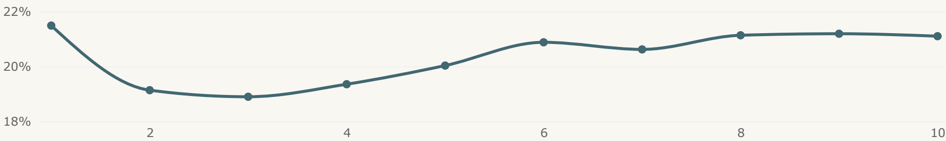
KSI % by IMD-decile
